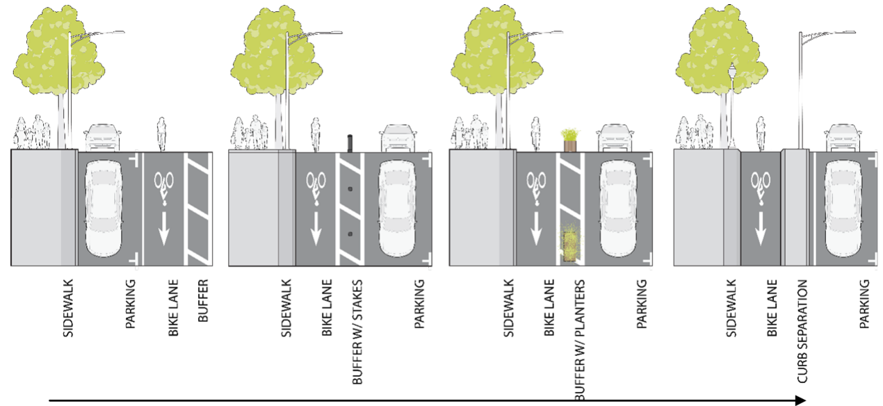
A typical design progression from a buffered bike lane to permanent separated bike lane
