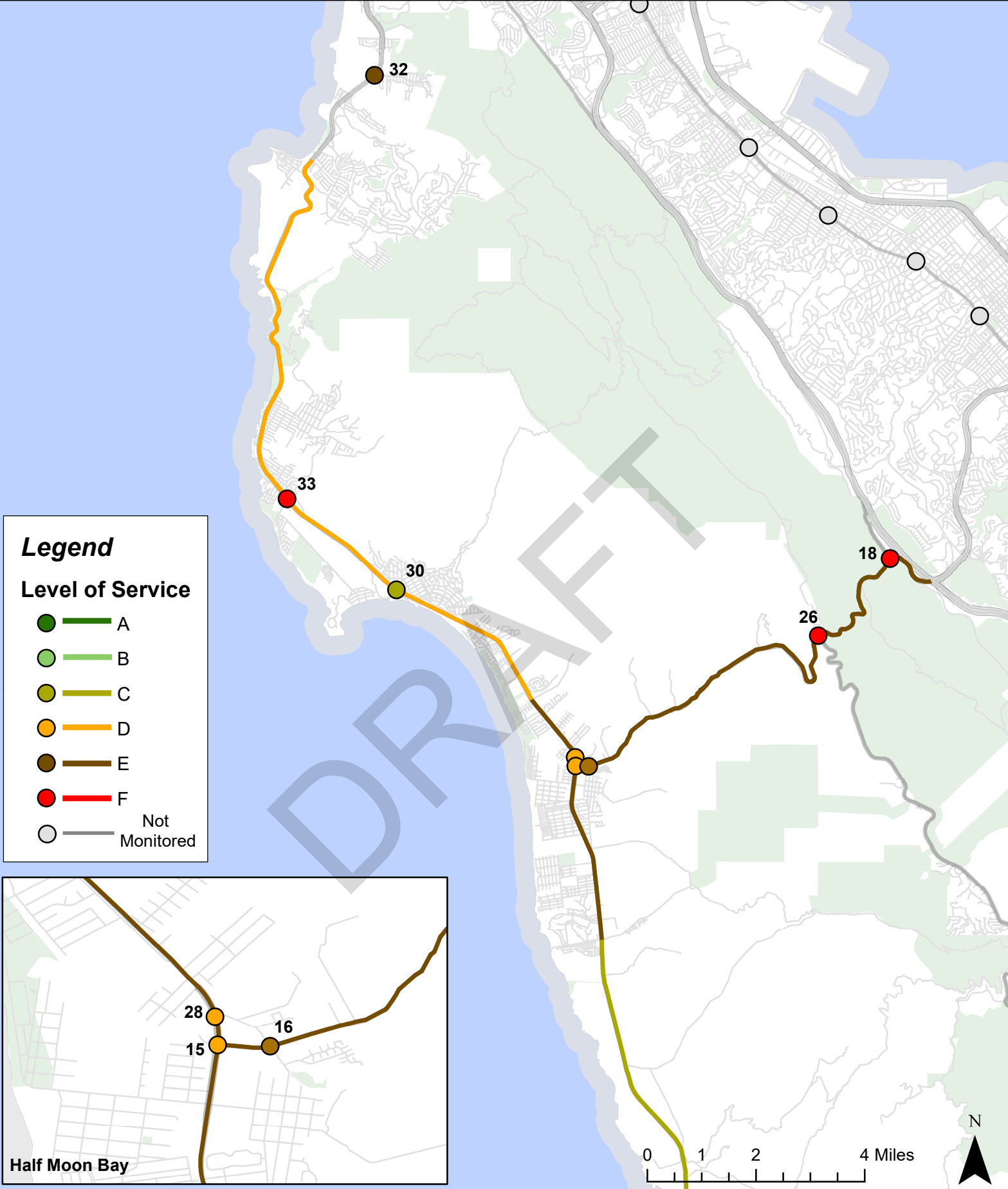
FIGURE 14 WEEKEND SEGMENT & INTERSECTION LOS MID-DAY PEAK PERIOD (2023) TJKM C/CAG City/County Association of Governments of San Mateo County
